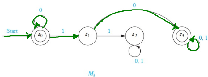
FIGURE 2 Some Finite-State Automata.
